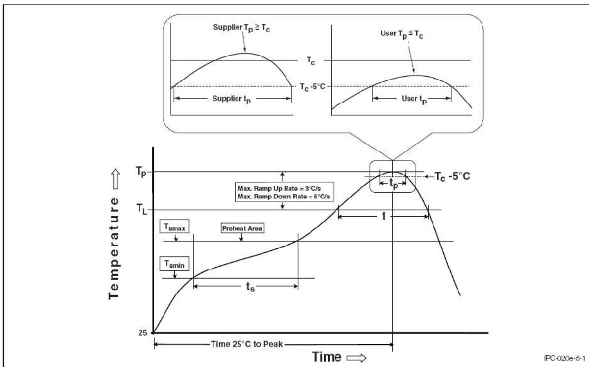
Soldering profile
