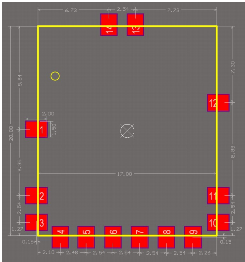
Footprint RTX-24EM-HPS-AE
