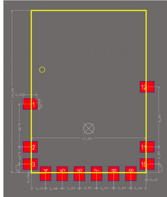
Footprint RTX-24EM-HPS-AI
