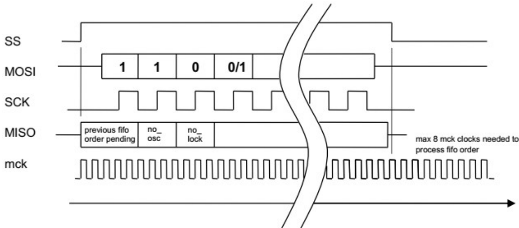
Figure 3: Timing of the SPI Read_RXFIFO / Write_TXFIFO command
