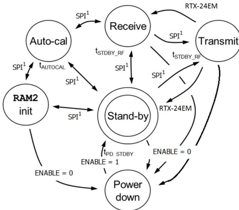
Figure 1: RTX-24EM-HPS-Ax Functional Overview
